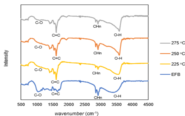
Figure 1 FT-IR spectrum of empty fruit bunch and biochar
